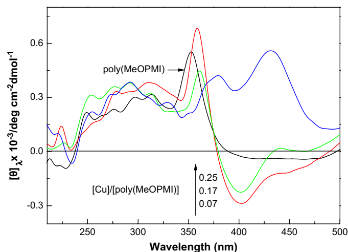
Fig. 5. CD spectral changes of poly(MeOPMI) (run 12 in Table 1, [\alpha]_D^{25} = +24.3^\circ ) in the presence of Cu(OTf) 2 in THF at ambient temperature with a polymer concentration of 1.0 mg mL -1 .
